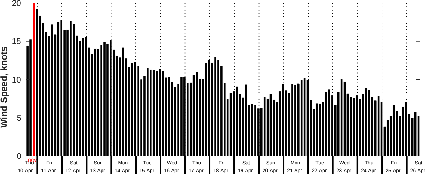
GFS Wind Speed Forecast for NDBC 51209 from 10-Apr-2025 13:00:00 to 26-Apr-2025 13:00:00
