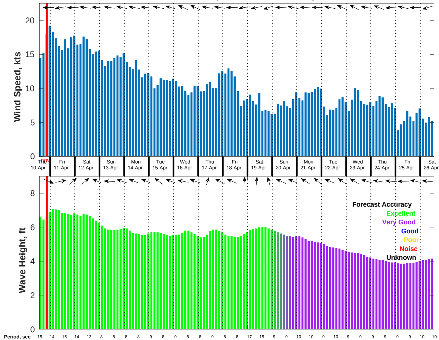
Wind & Wave Forecast for NDBC 51209 from 10-Apr-2025 13:00:00 to 26-Apr-2025 13:00:00
