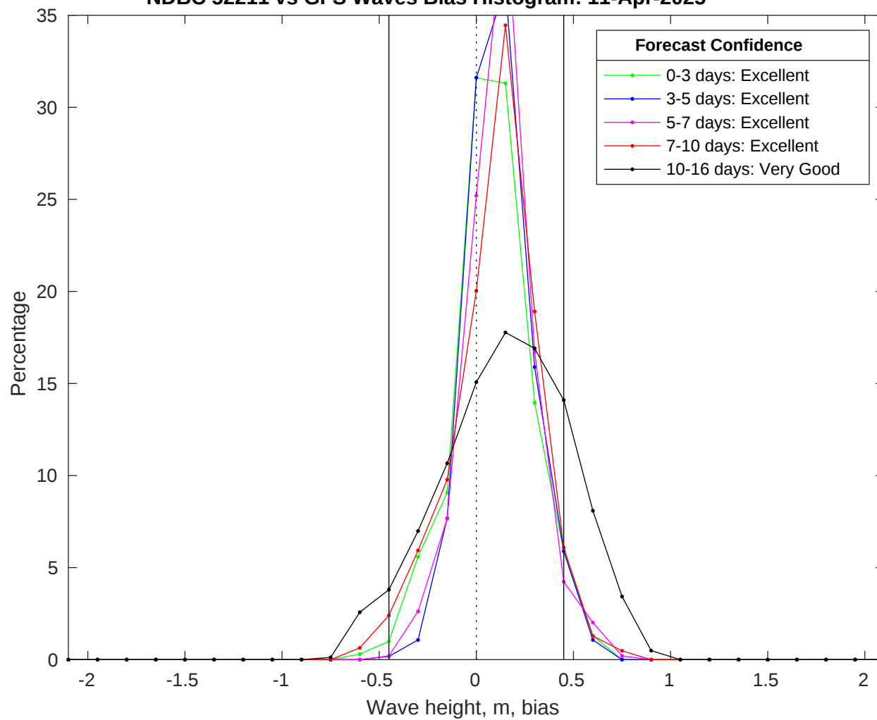
NDBC 52211 vs GFS Waves Bias Histogram: 11-Apr-2025
