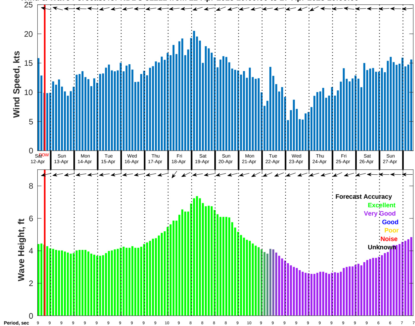
Wind & Wave Forecast for NDBC 52211 from 11-Apr-2025 10:00:00 to 27-Apr-2025 10:00:00
