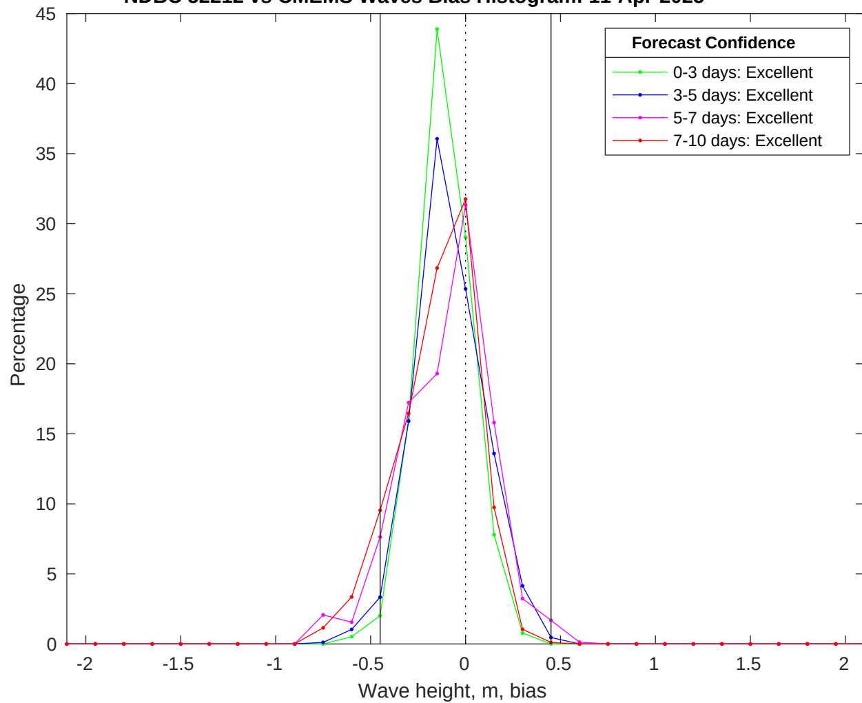
NDBC 52212 vs CMEMS Waves Bias Histogram: 11-Apr-2025
