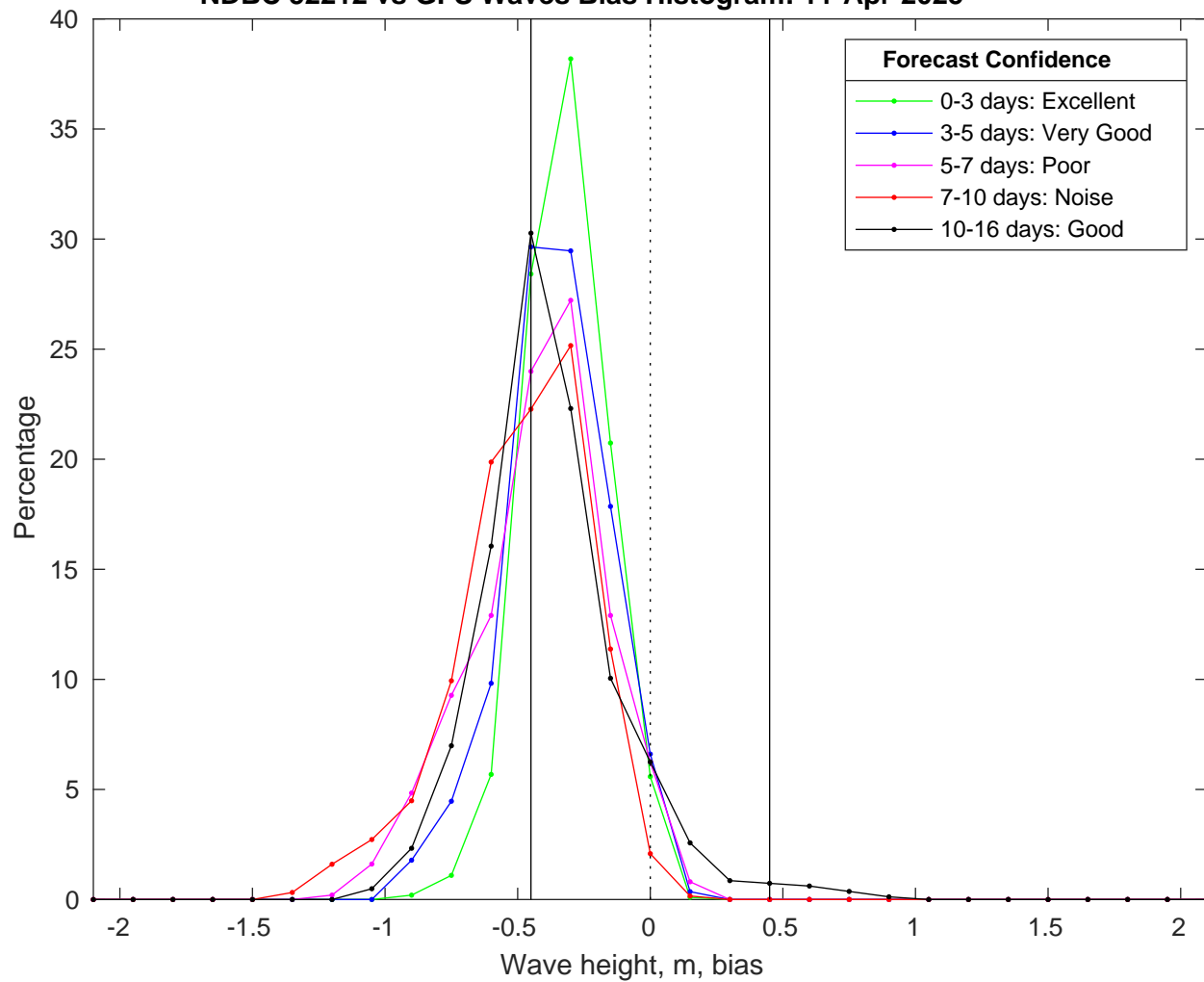
NDBC 52212 vs GFS Waves Bias Histogram: 11-Apr-2025
