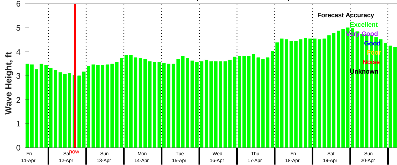
CMEMS Wave Forecast for NDBC 52212 from 10-Apr-2025 09:00:00 to 20-Apr-2025 09:00:00
