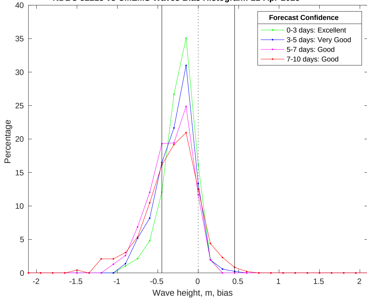
NDBC 52213 vs CMEMS Waves Bias Histogram: 11-Apr-2025
