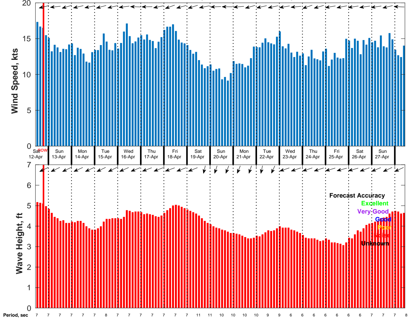
Wind & Wave Forecast for NDBC 52213 from 11-Apr-2025 11:00:00 to 27-Apr-2025 11:00:00
