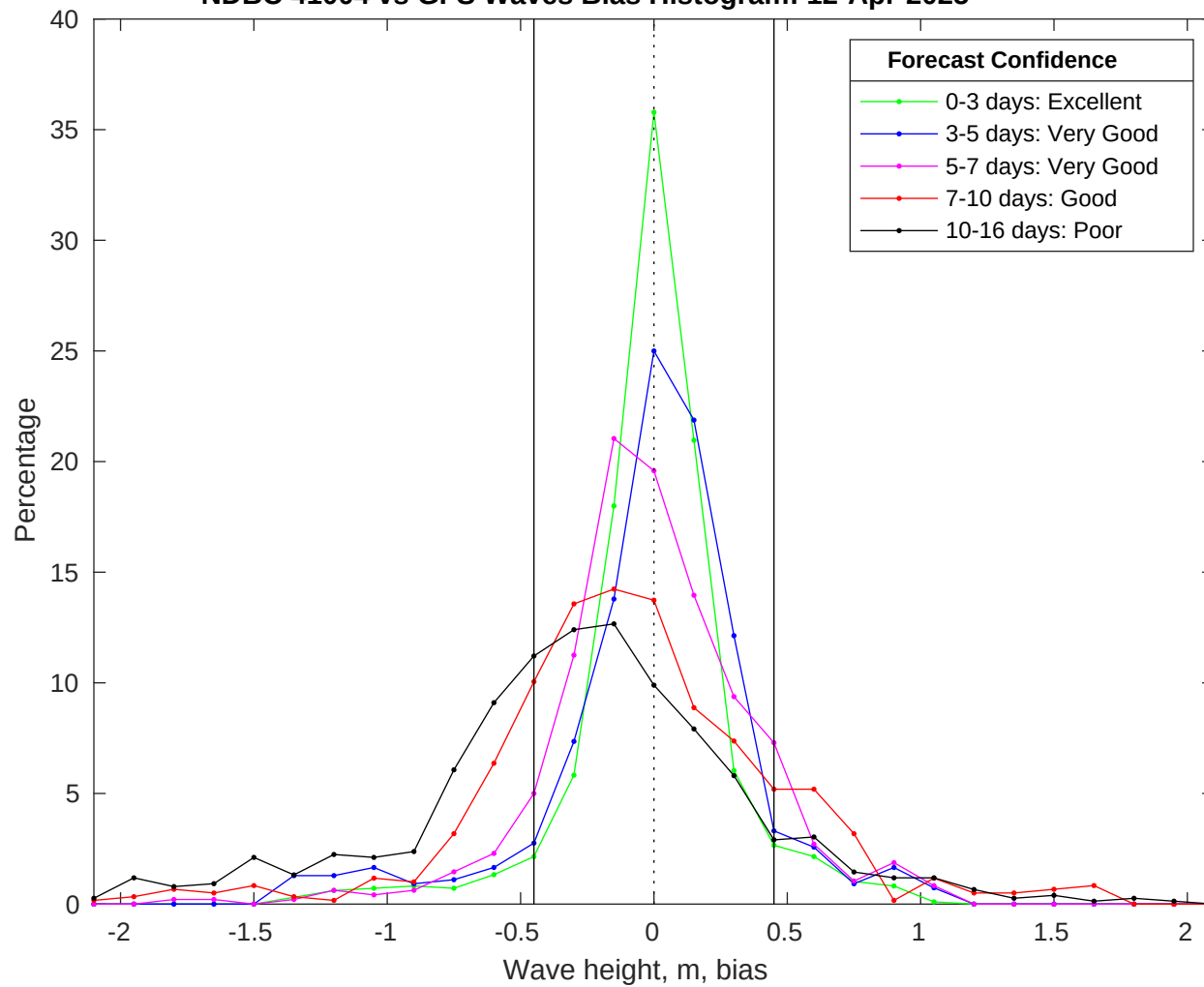
NDBC 41004 vs GFS Waves Bias Histogram: 12-Apr-2025
