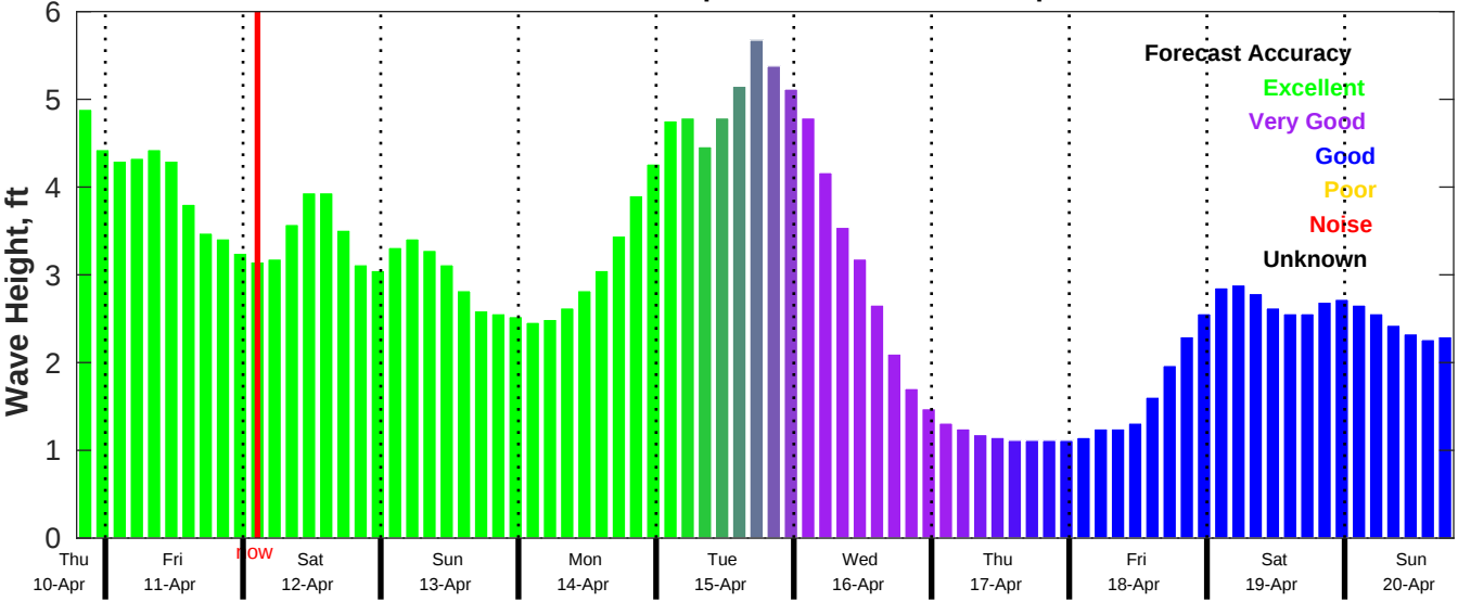
CMEMS Wave Forecast for NDBC 41004 from 10-Apr-2025 19:00:00 to 20-Apr-2025 19:00:00
