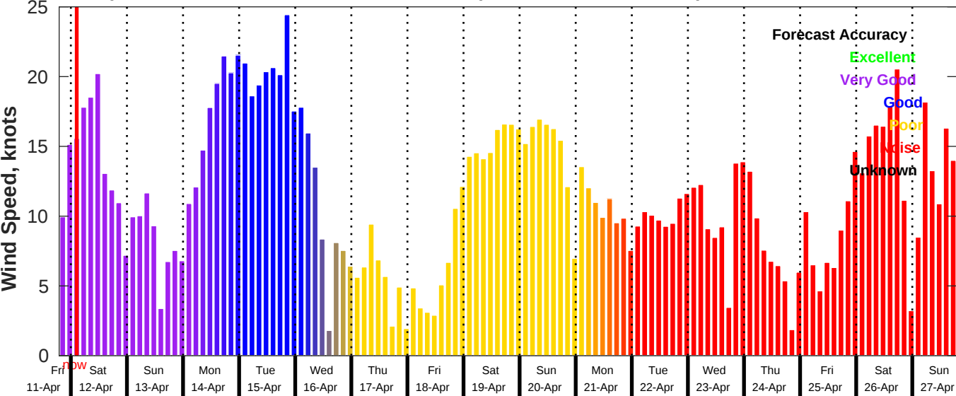
GFS Wind Speed Forecast for NDBC 41004 from 11-Apr-2025 19:00:00 to 27-Apr-2025 19:00:00
