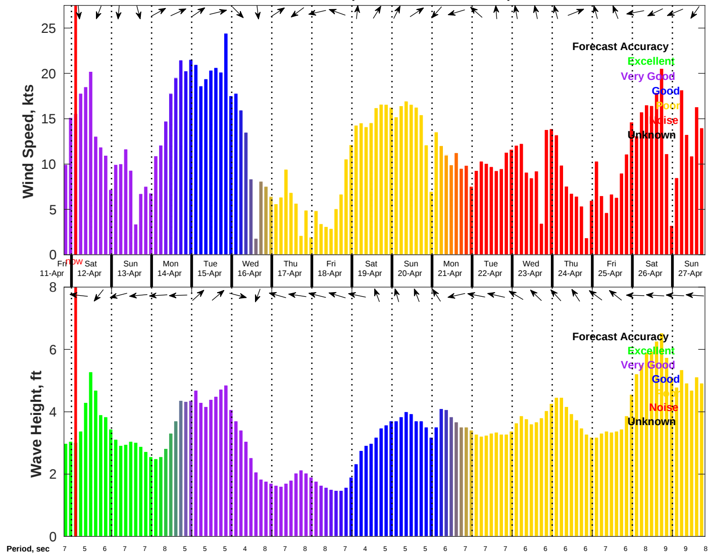
Wind & Wave Forecast for NDBC 41004 from 11-Apr-2025 19:00:00 to 27-Apr-2025 19:00:00
