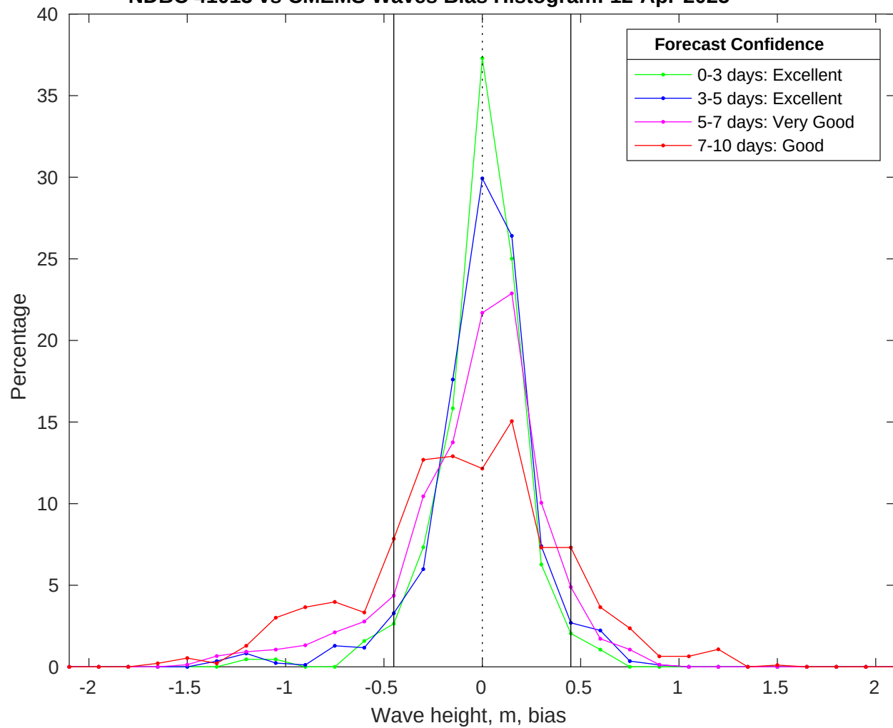
NDBC 41013 vs CMEMS Waves Bias Histogram: 12-Apr-2025
