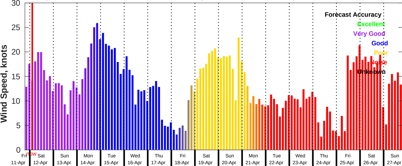
GFS Wind Speed Forecast for NDBC 41013 from 11-Apr-2025 19:00:00 to 27-Apr-2025 19:00:00
