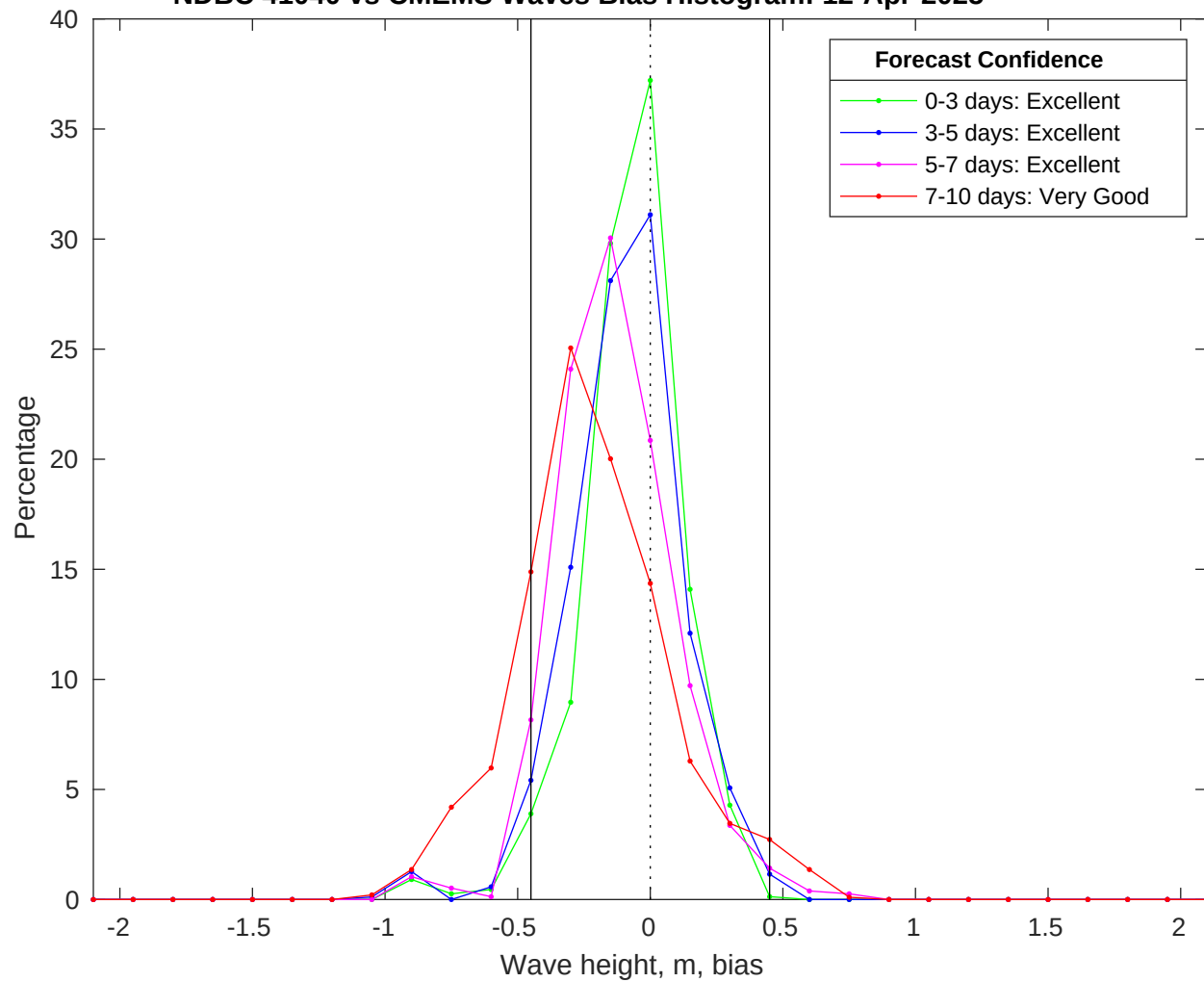
NDBC 41040 vs CMEMS Waves Bias Histogram: 12-Apr-2025
