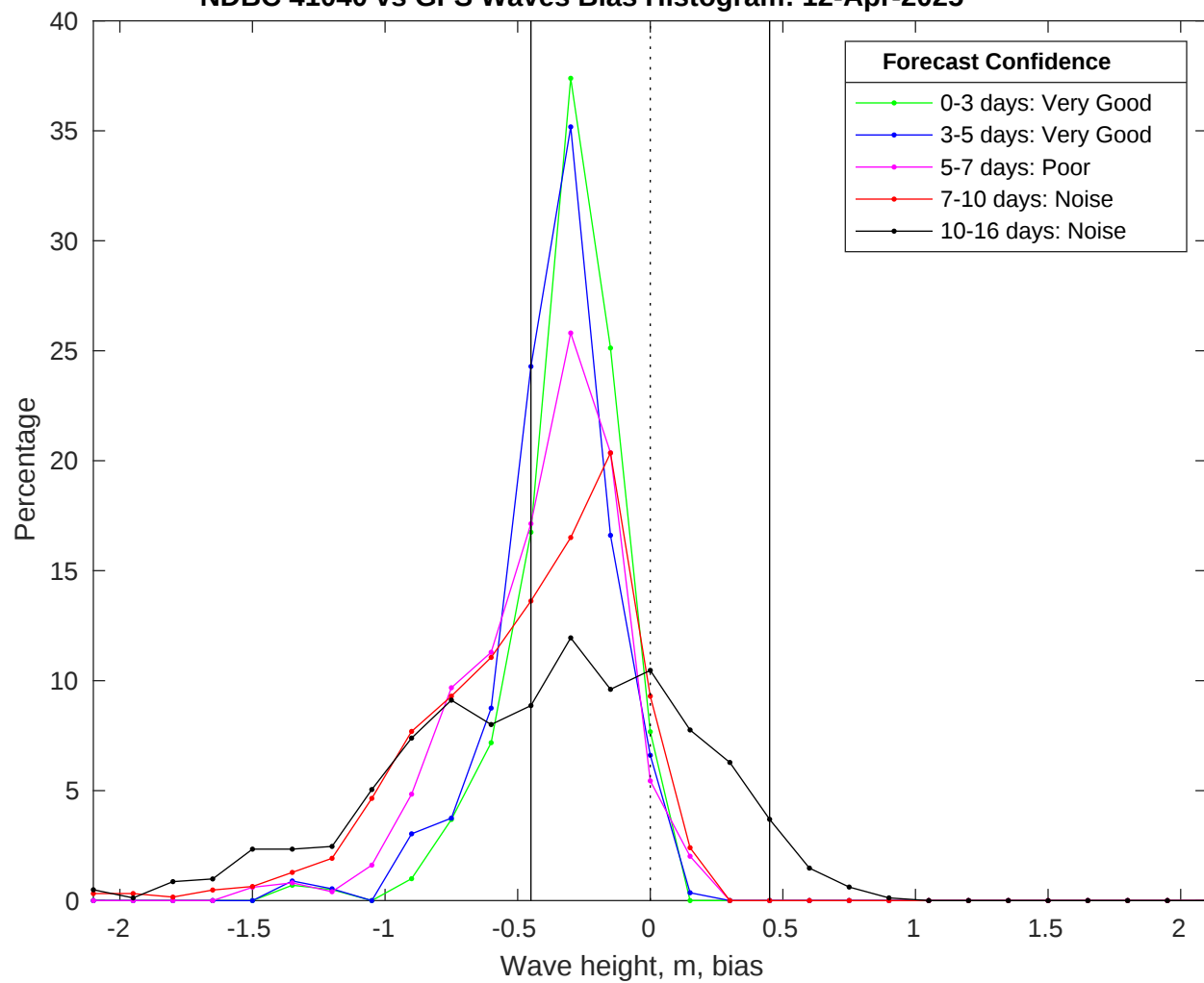
NDBC 41040 vs GFS Waves Bias Histogram: 12-Apr-2025
