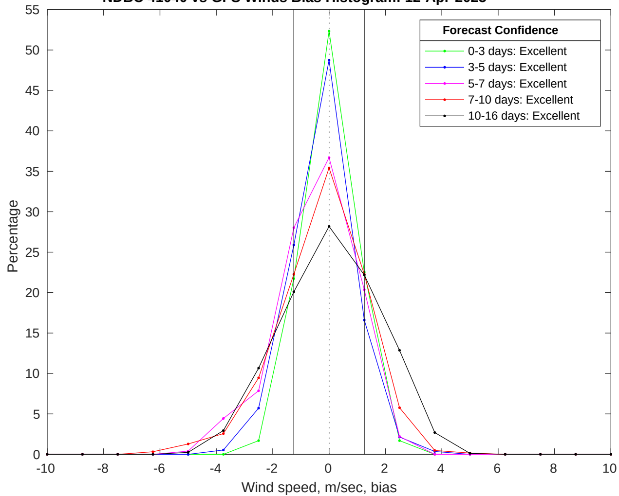
NDBC 41040 vs GFS Winds Bias Histogram: 12-Apr-2025
