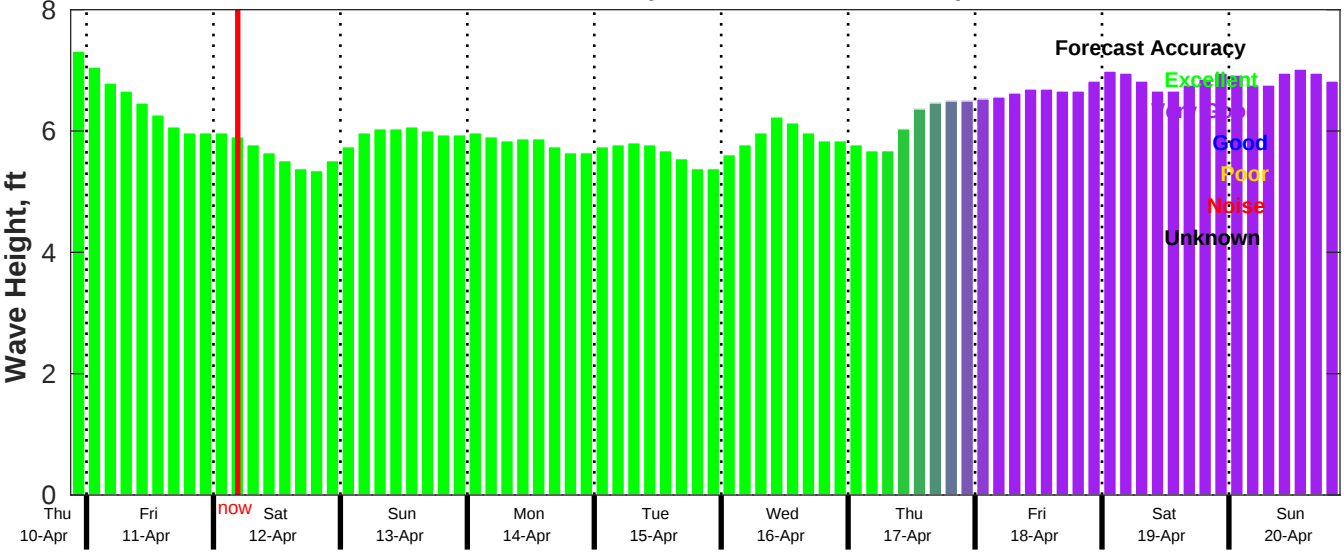
CMEMS Wave Forecast for NDBC 41040 from 10-Apr-2025 21:00:00 to 20-Apr-2025 21:00:00
