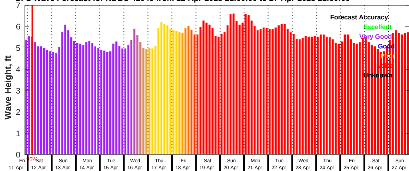
GFS Wave Forecast for NDBC 41040 from 11-Apr-2025 21:00:00 to 27-Apr-2025 21:00:00
