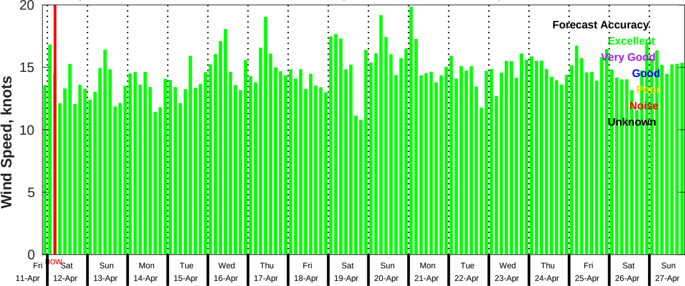
GFS Wind Speed Forecast for NDBC 41040 from 11-Apr-2025 21:00:00 to 27-Apr-2025 21:00:00
