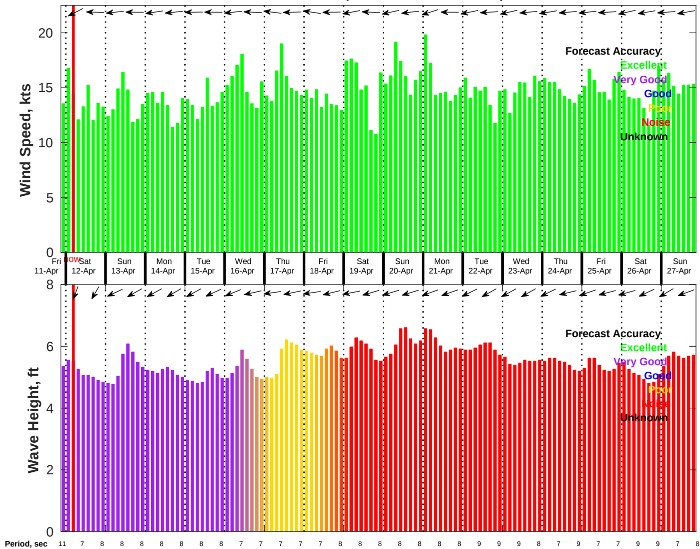
Wind & Wave Forecast for NDBC 41040 from 11-Apr-2025 21:00:00 to 27-Apr-2025 21:00:00
