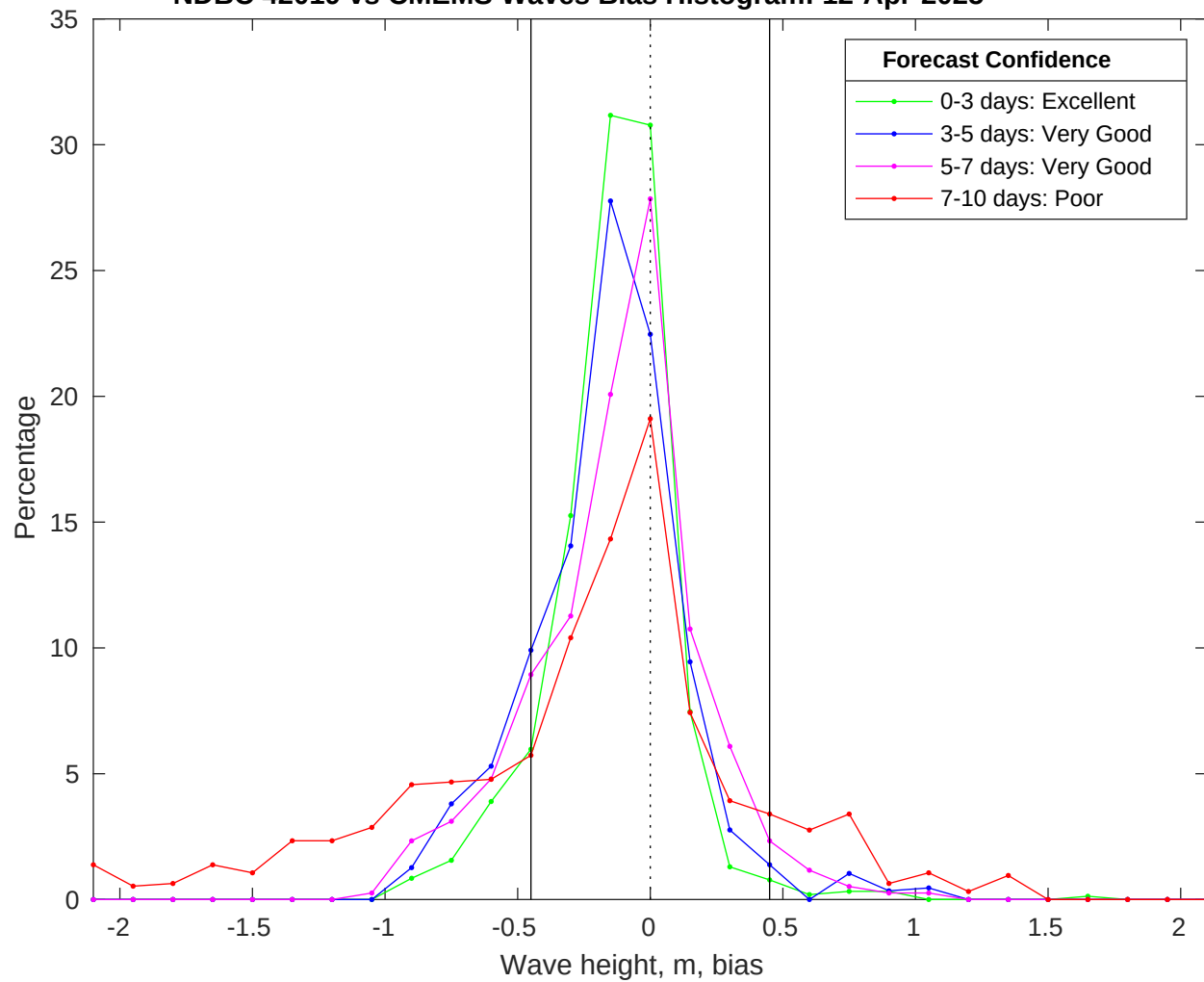
NDBC 42019 vs CMEMS Waves Bias Histogram: 12-Apr-2025
