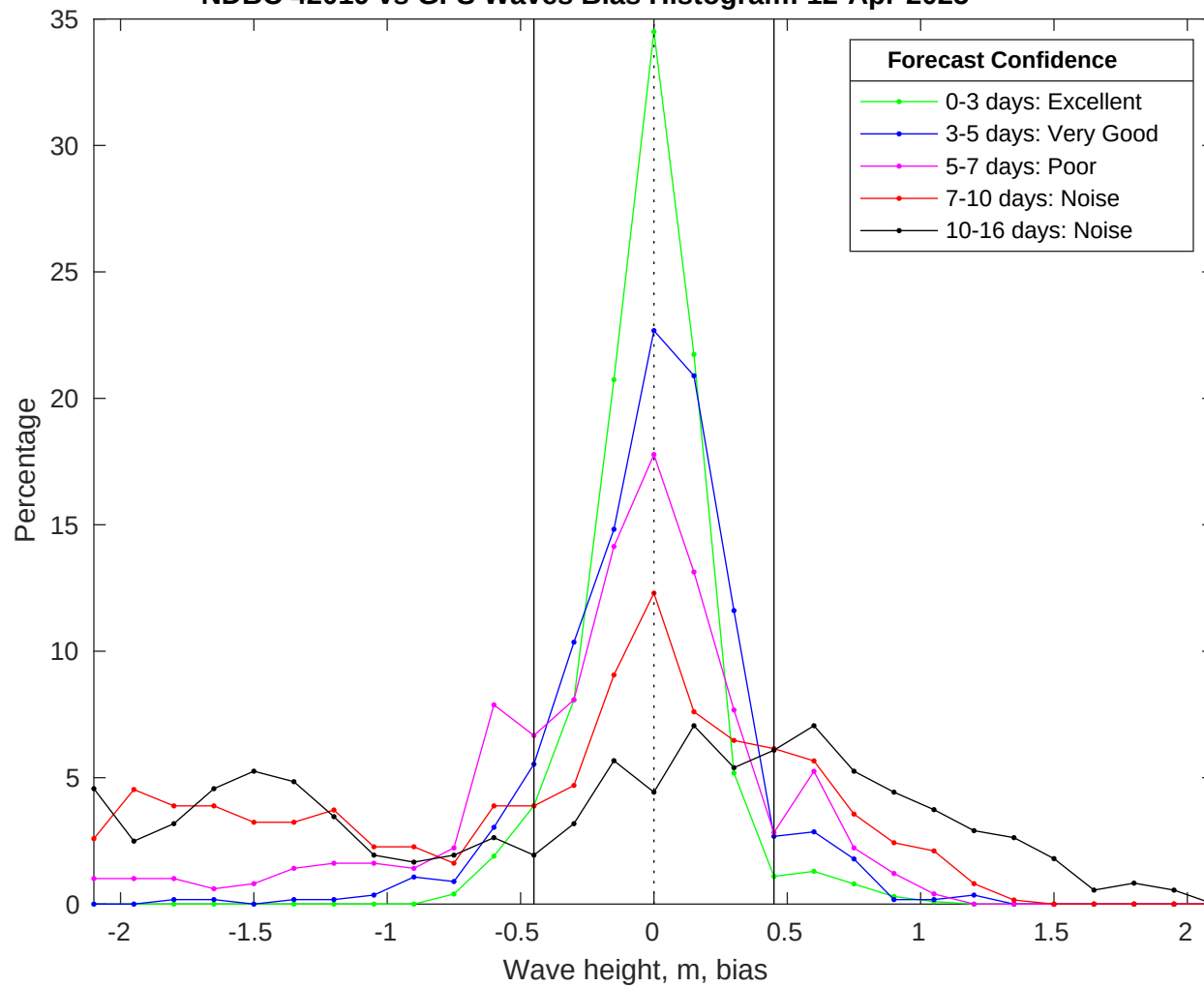
NDBC 42019 vs GFS Waves Bias Histogram: 12-Apr-2025
