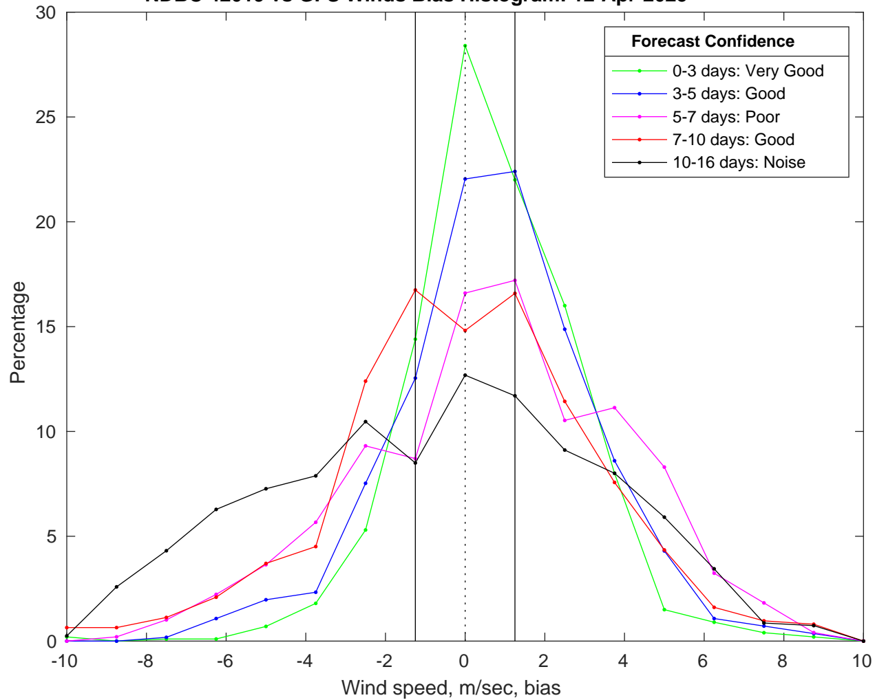
NDBC 42019 vs GFS Winds Bias Histogram: 12-Apr-2025
