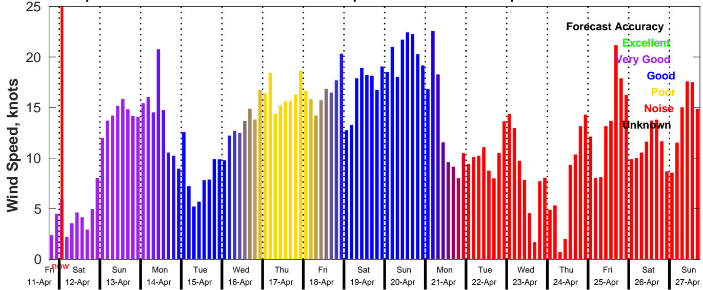
GFS Wind Speed Forecast for NDBC 42019 from 11-Apr-2025 18:00:00 to 27-Apr-2025 18:00:00
