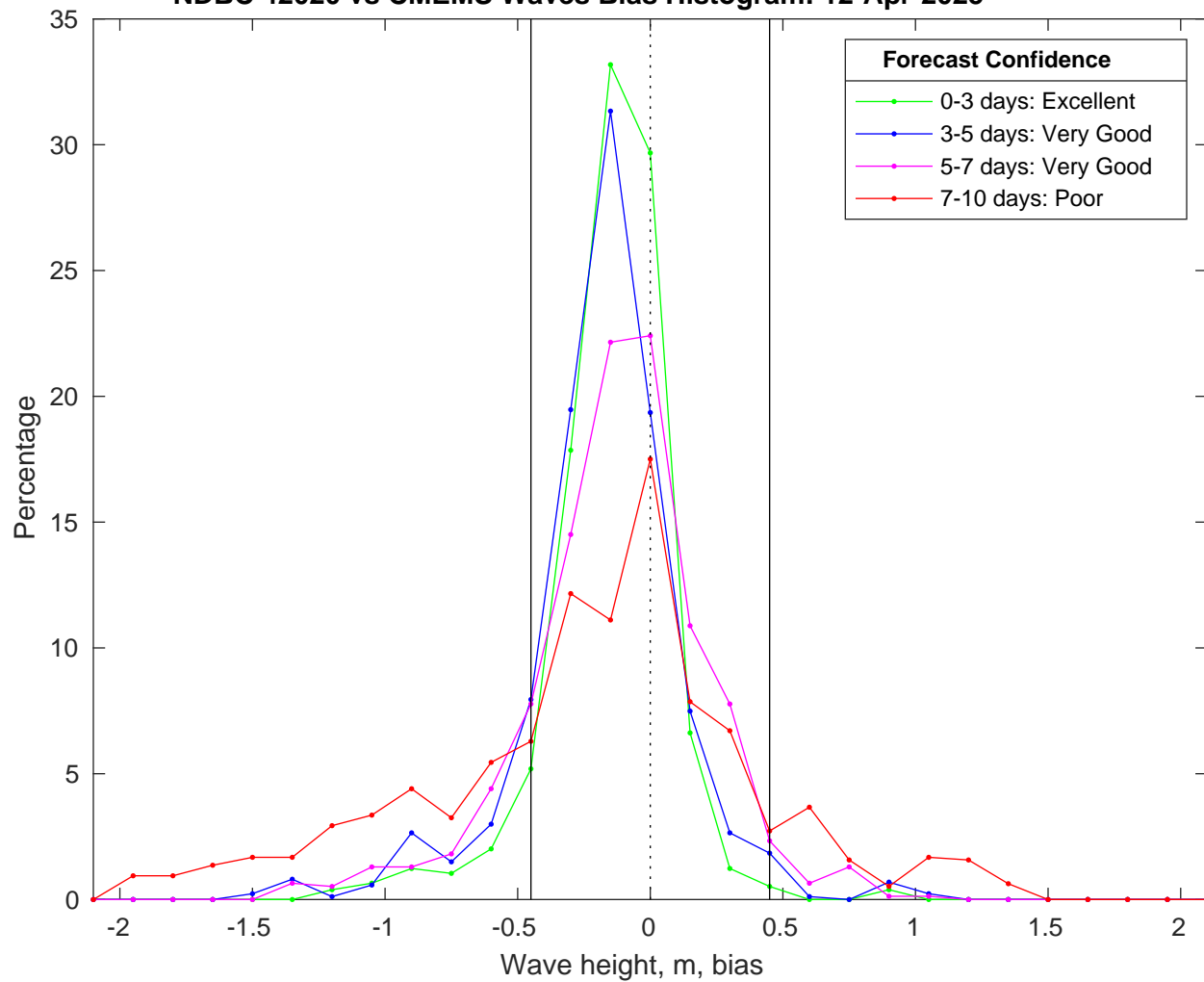
NDBC 42020 vs CMEMS Waves Bias Histogram: 12-Apr-2025
