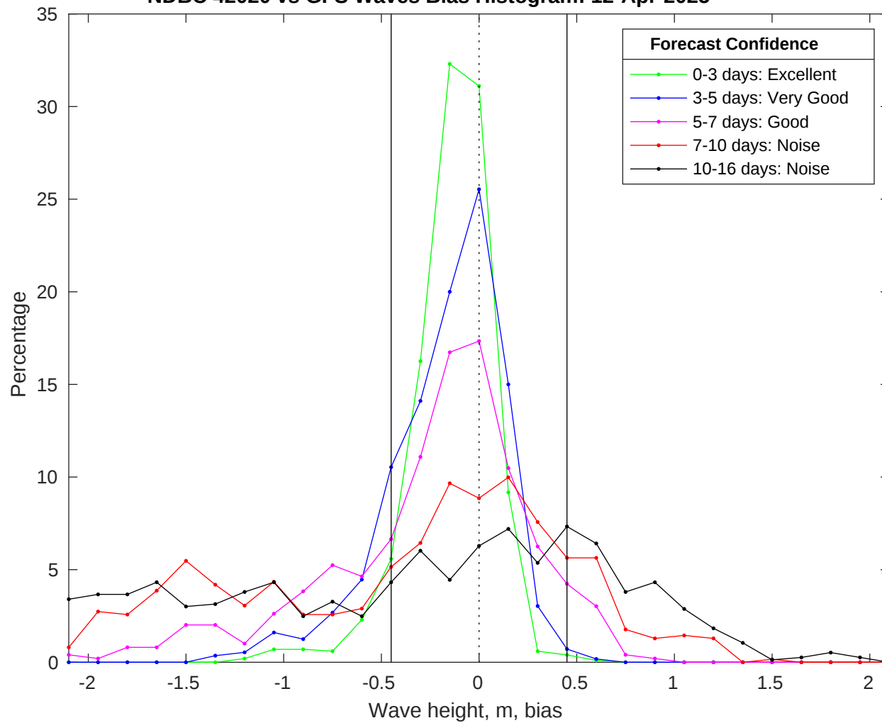
NDBC 42020 vs GFS Waves Bias Histogram: 12-Apr-2025
