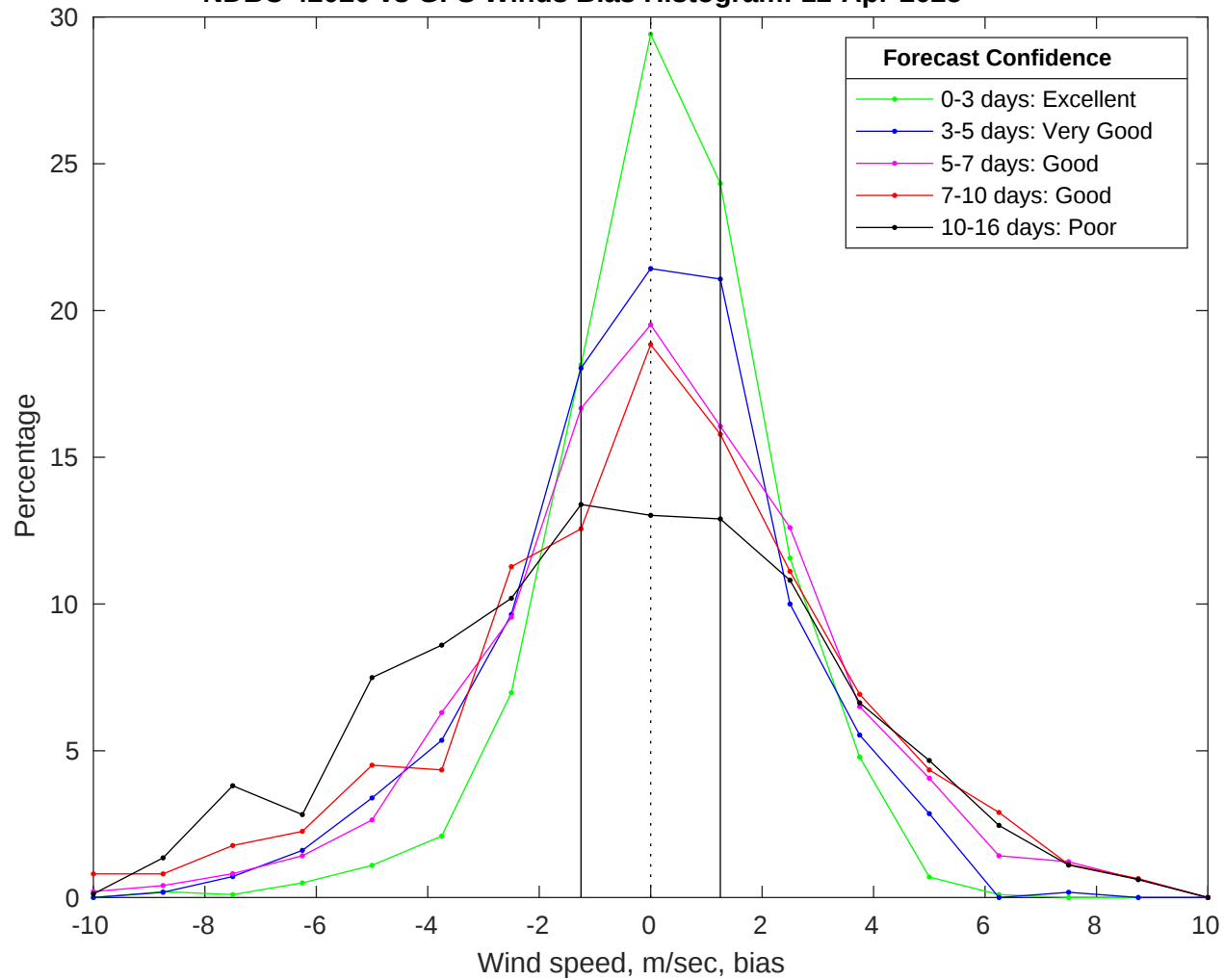
NDBC 42020 vs GFS Winds Bias Histogram: 12-Apr-2025
