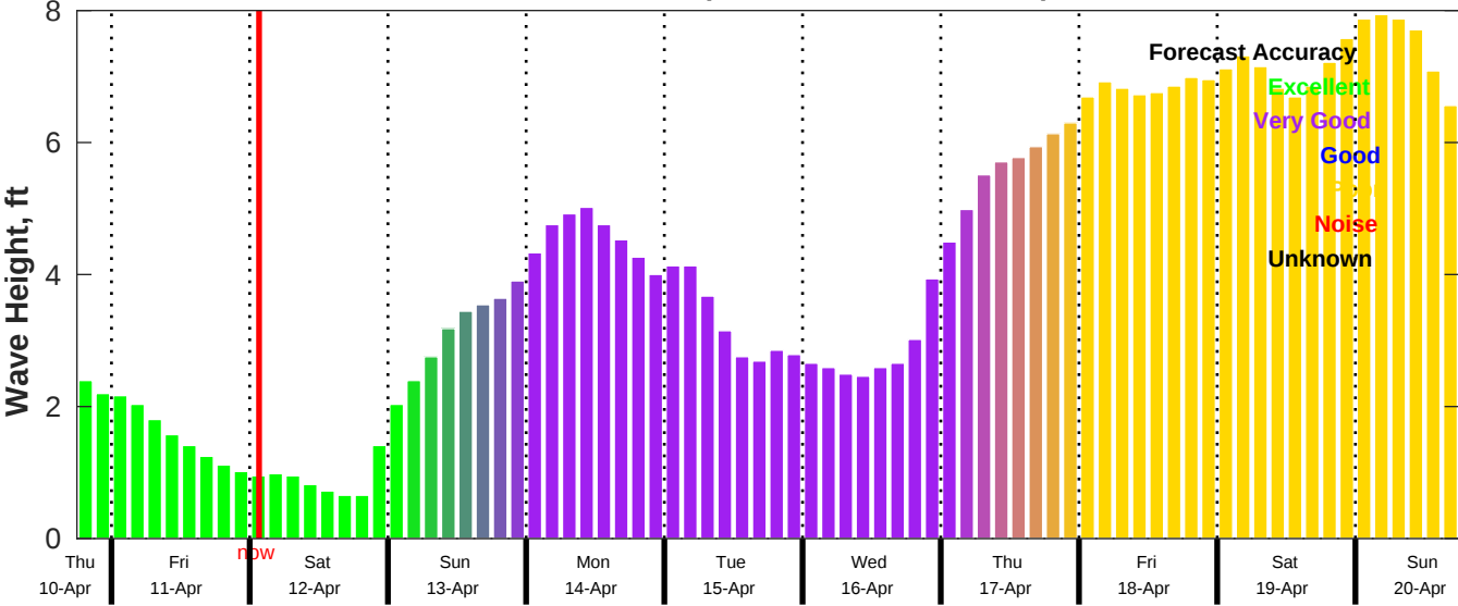
CMEMS Wave Forecast for NDBC 42020 from 10-Apr-2025 18:00:00 to 20-Apr-2025 18:00:00
