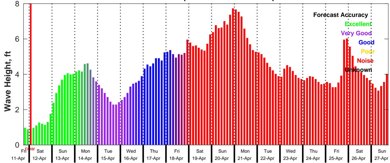
GFS Wave Forecast for NDBC 42020 from 11-Apr-2025 18:00:00 to 27-Apr-2025 18:00:00
