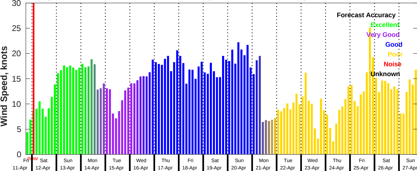
GFS Wind Speed Forecast for NDBC 42020 from 11-Apr-2025 18:00:00 to 27-Apr-2025 18:00:00
