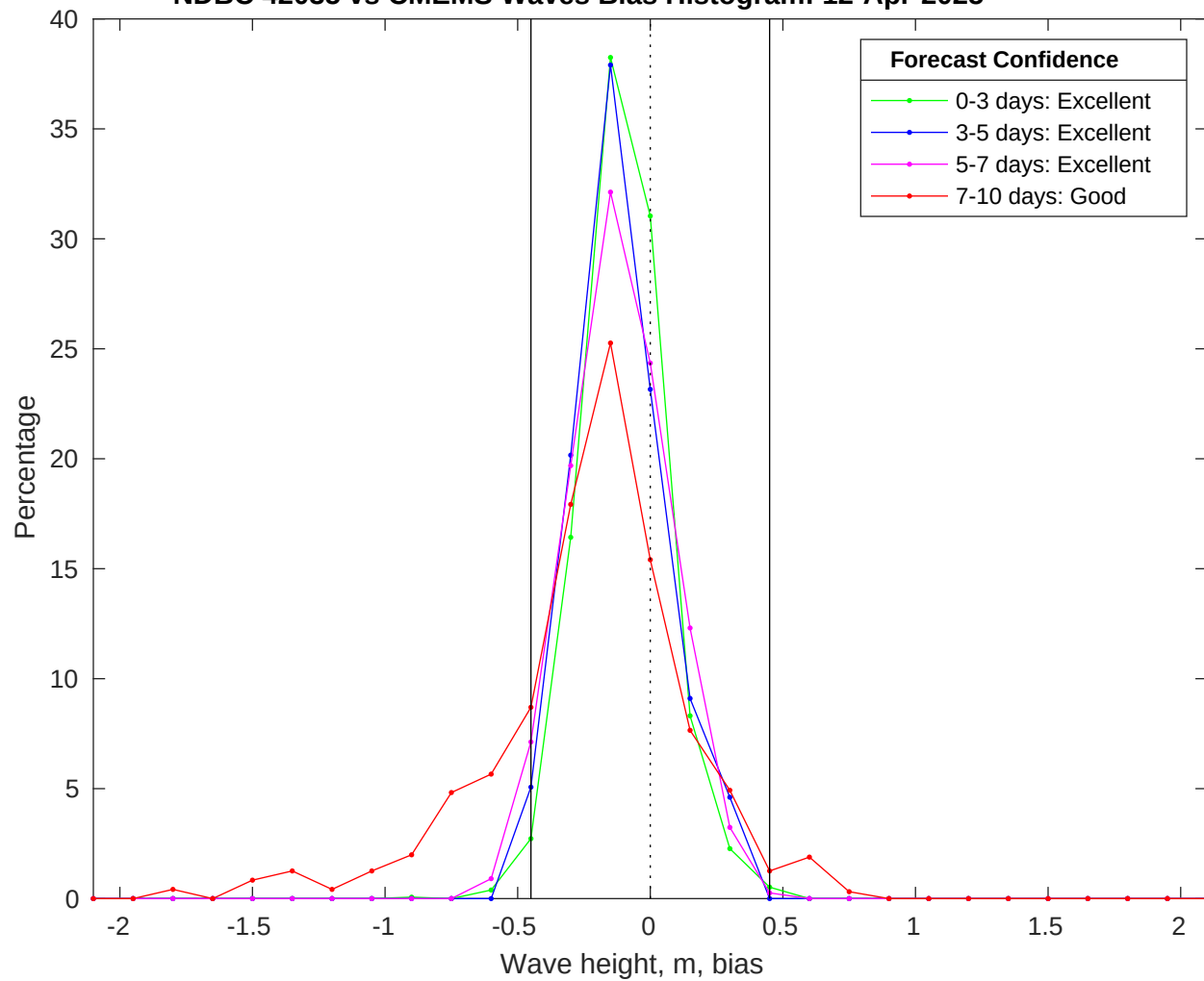
NDBC 42035 vs CMEMS Waves Bias Histogram: 12-Apr-2025
