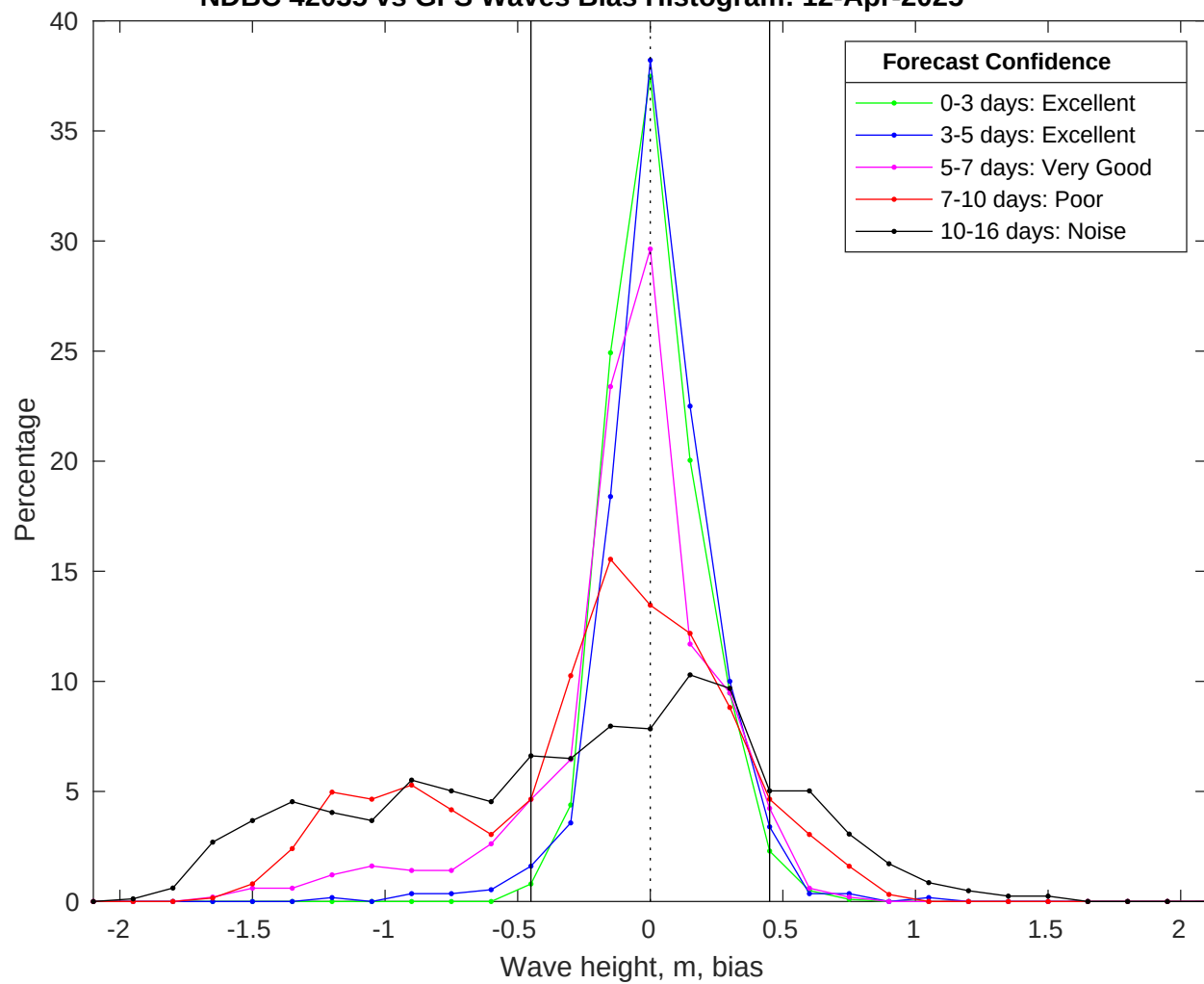
NDBC 42035 vs GFS Waves Bias Histogram: 12-Apr-2025
