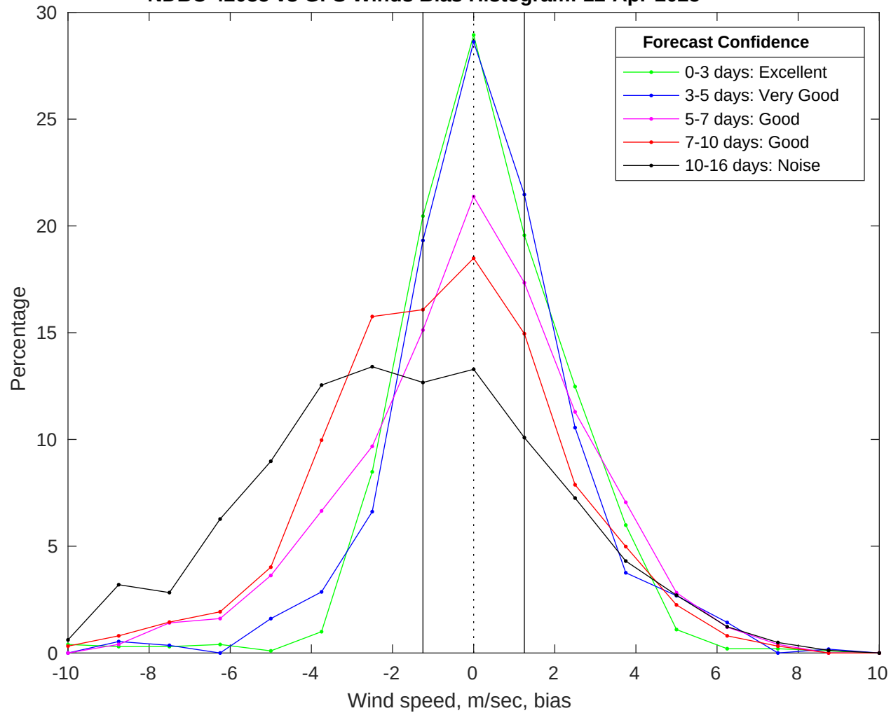
NDBC 42035 vs GFS Winds Bias Histogram: 12-Apr-2025
