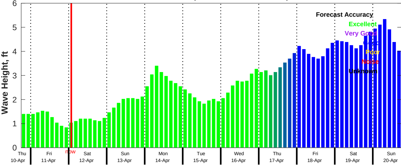
CMEMS Wave Forecast for NDBC 42035 from 10-Apr-2025 18:00:00 to 20-Apr-2025 18:00:00
