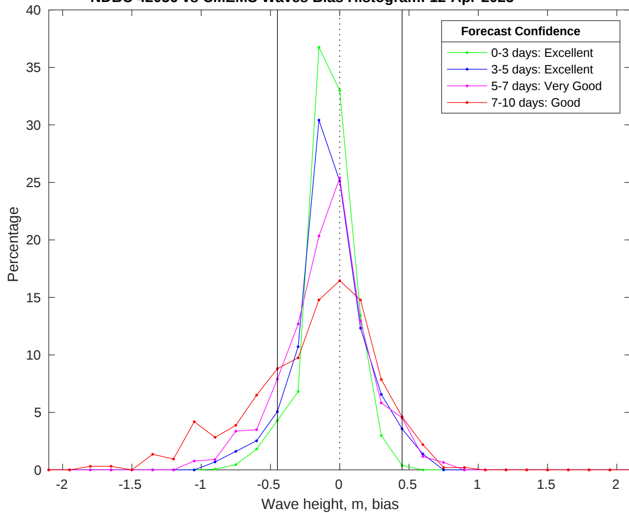
NDBC 42036 vs CMEMS Waves Bias Histogram: 12-Apr-2025
