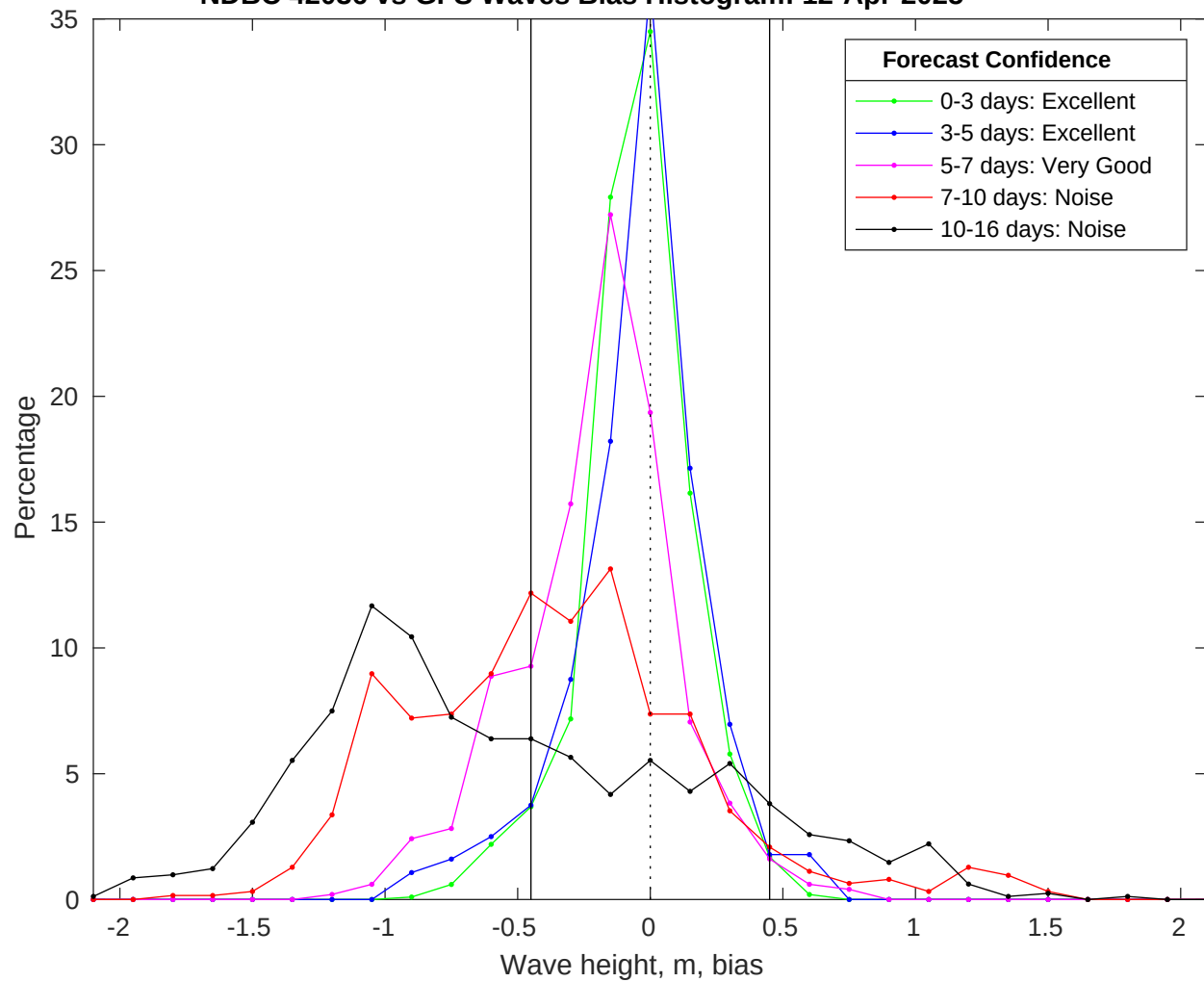
NDBC 42036 vs GFS Waves Bias Histogram: 12-Apr-2025
