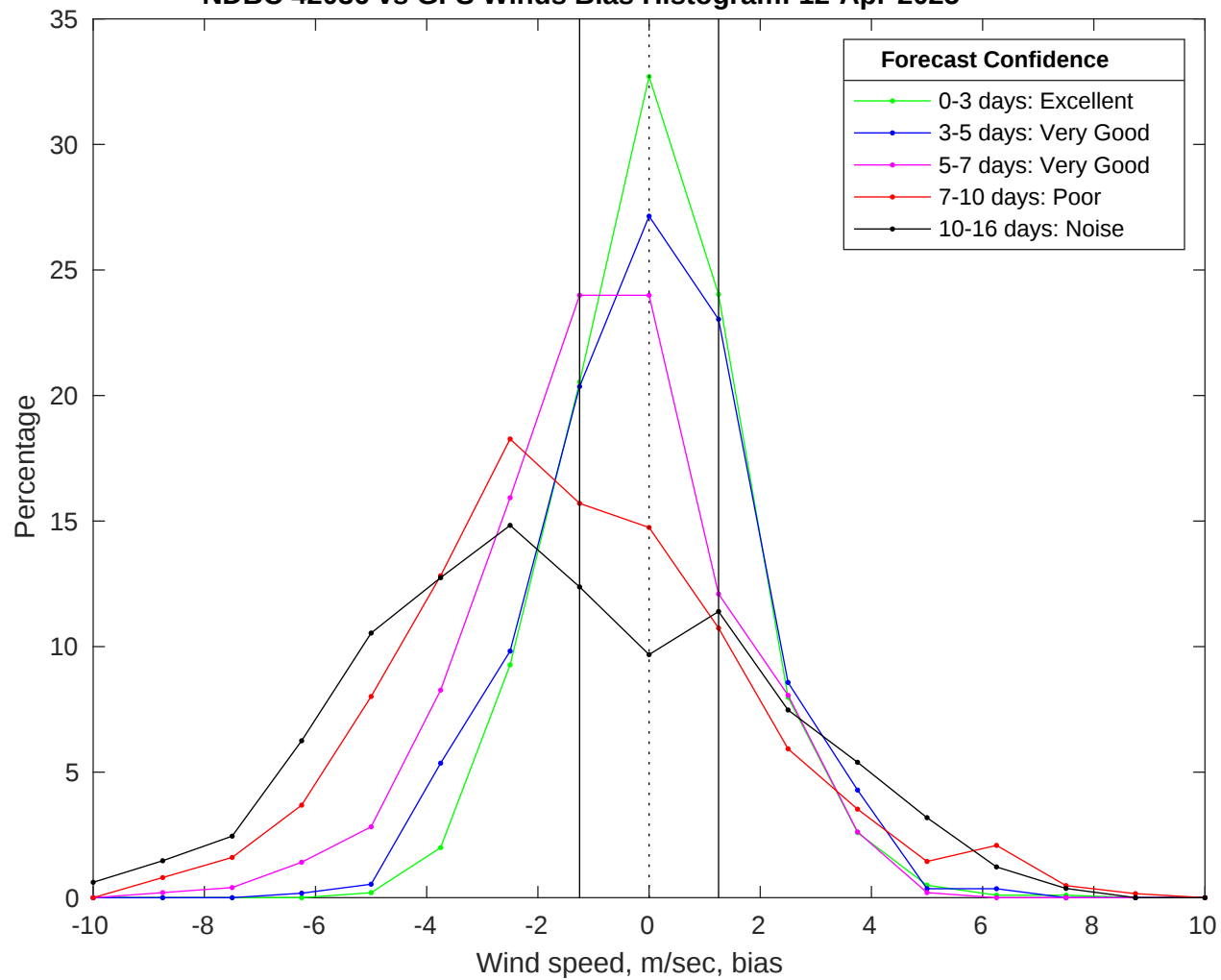
NDBC 42036 vs GFS Winds Bias Histogram: 12-Apr-2025
