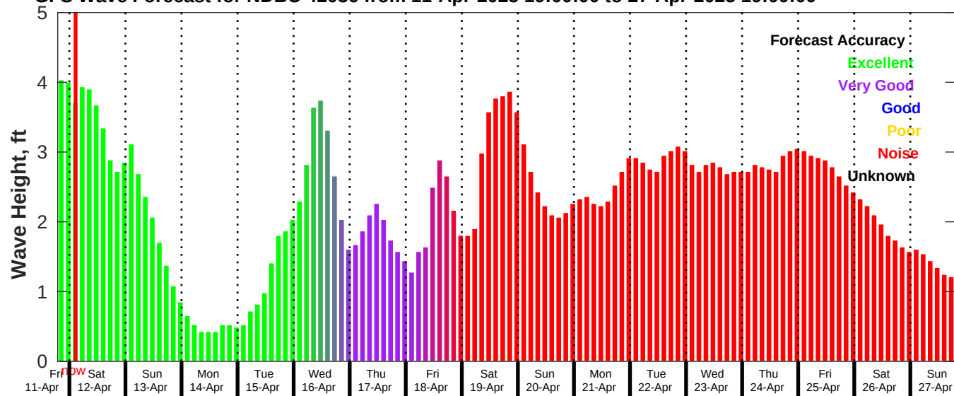
GFS Wave Forecast for NDBC 42036 from 11-Apr-2025 19:00:00 to 27-Apr-2025 19:00:00
