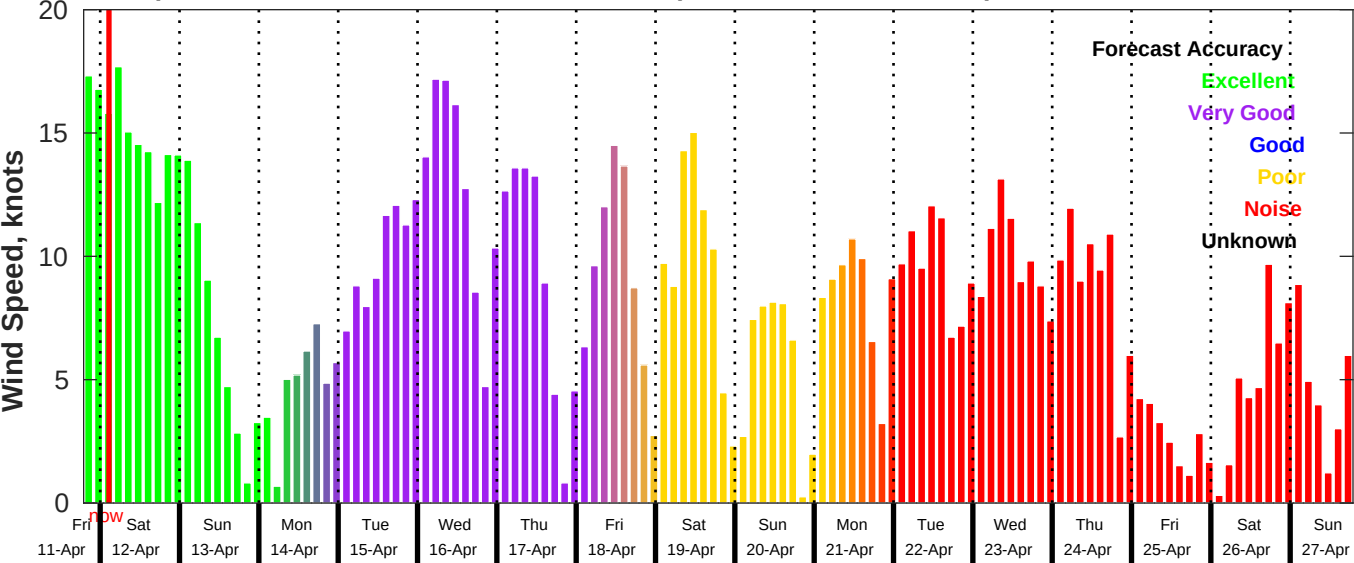
GFS Wind Speed Forecast for NDBC 42036 from 11-Apr-2025 19:00:00 to 27-Apr-2025 19:00:00
