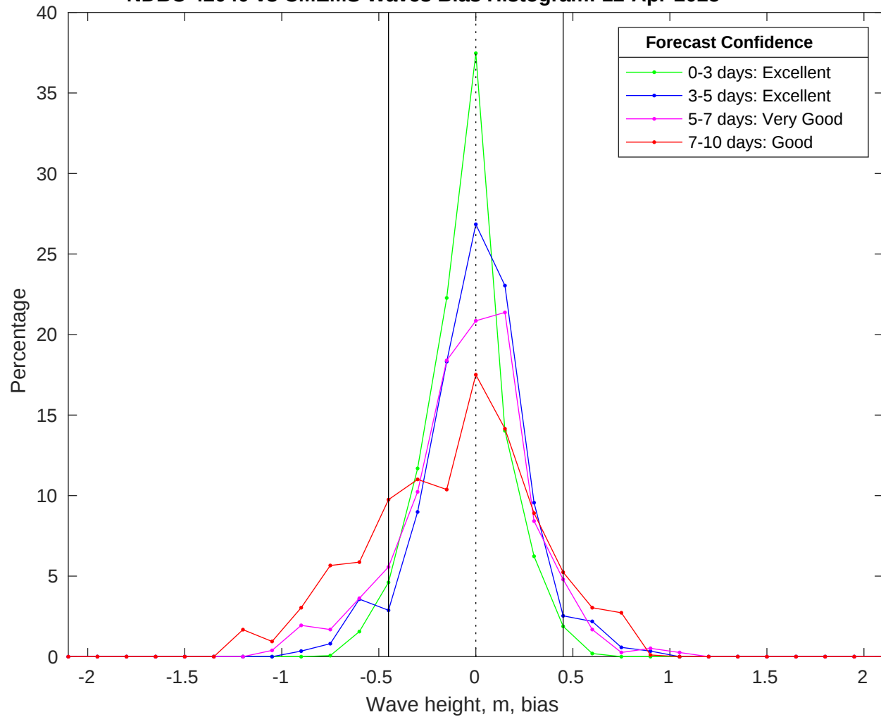
NDBC 42040 vs CMEMS Waves Bias Histogram: 12-Apr-2025
