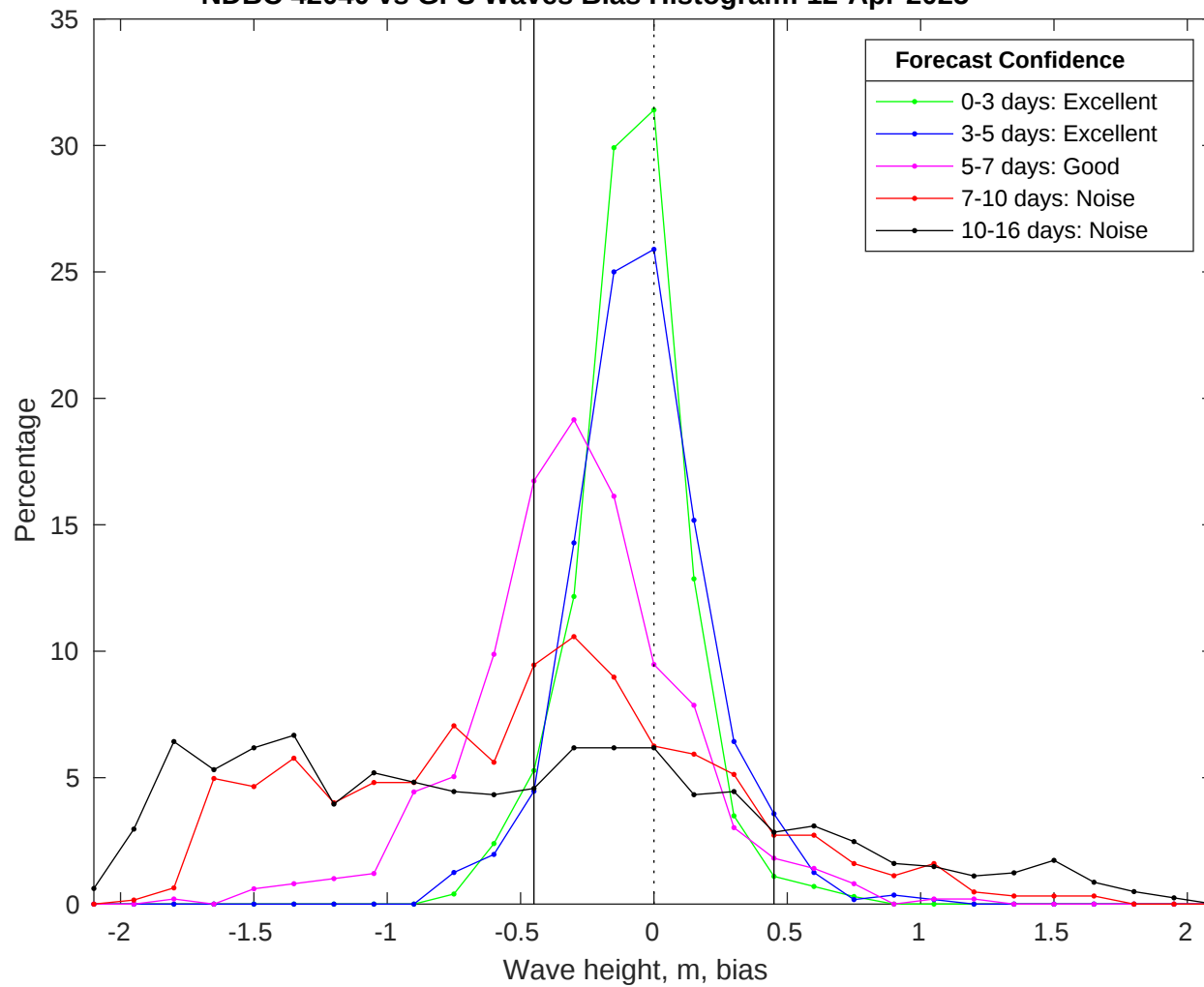
NDBC 42040 vs GFS Waves Bias Histogram: 12-Apr-2025
