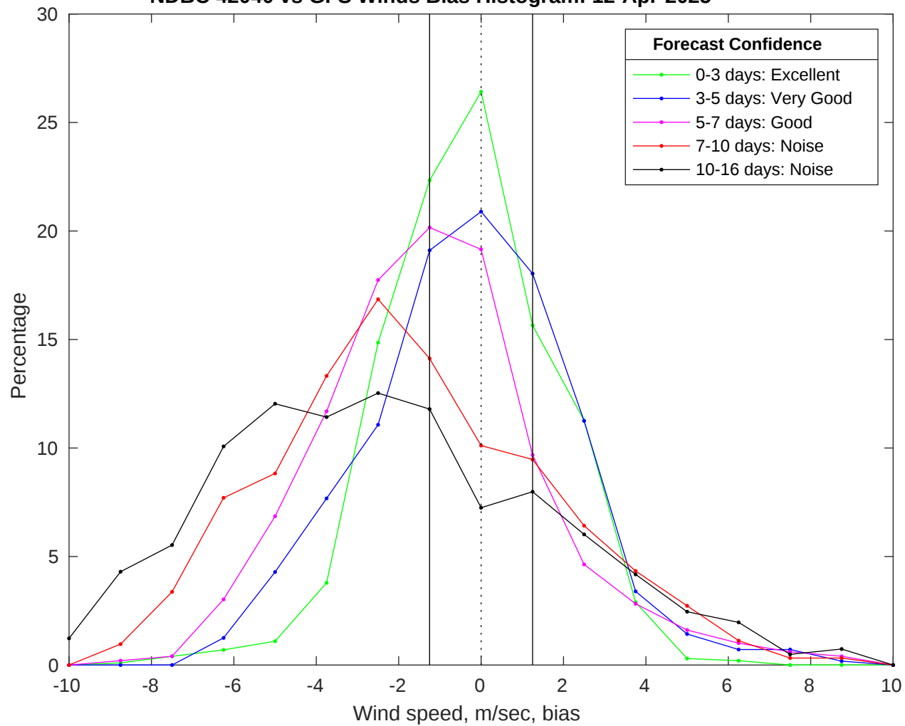
NDBC 42040 vs GFS Winds Bias Histogram: 12-Apr-2025
