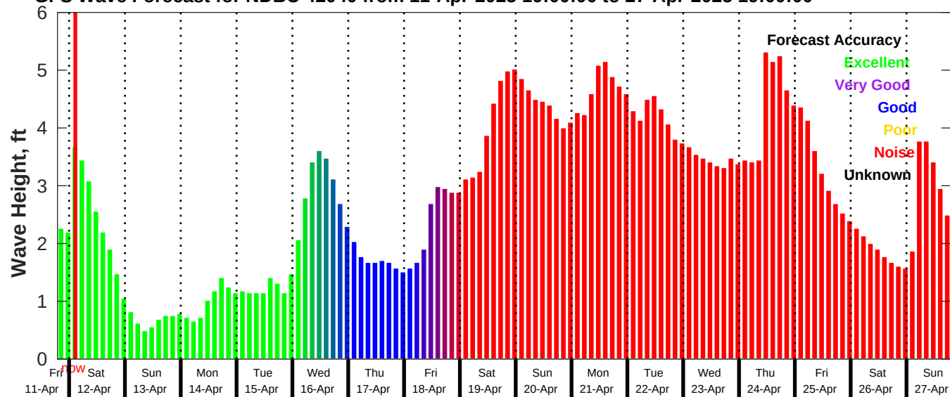
GFS Wave Forecast for NDBC 42040 from 11-Apr-2025 19:00:00 to 27-Apr-2025 19:00:00
