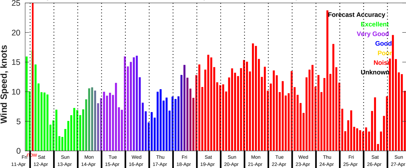
GFS Wind Speed Forecast for NDBC 42040 from 11-Apr-2025 19:00:00 to 27-Apr-2025 19:00:00
