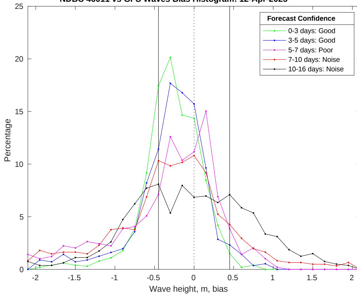
NDBC 46011 vs GFS Waves Bias Histogram: 12-Apr-2025
