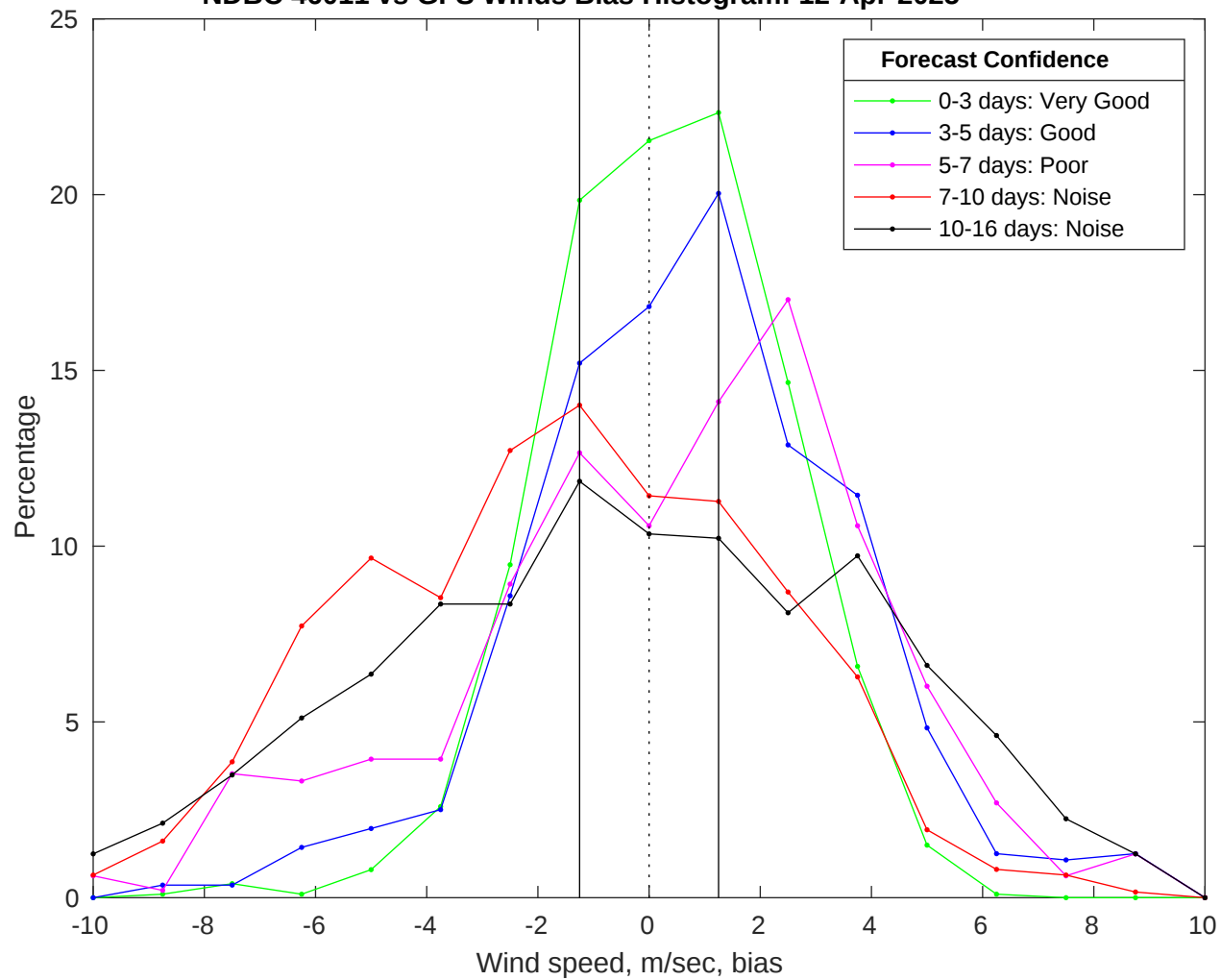
NDBC 46011 vs GFS Winds Bias Histogram: 12-Apr-2025
