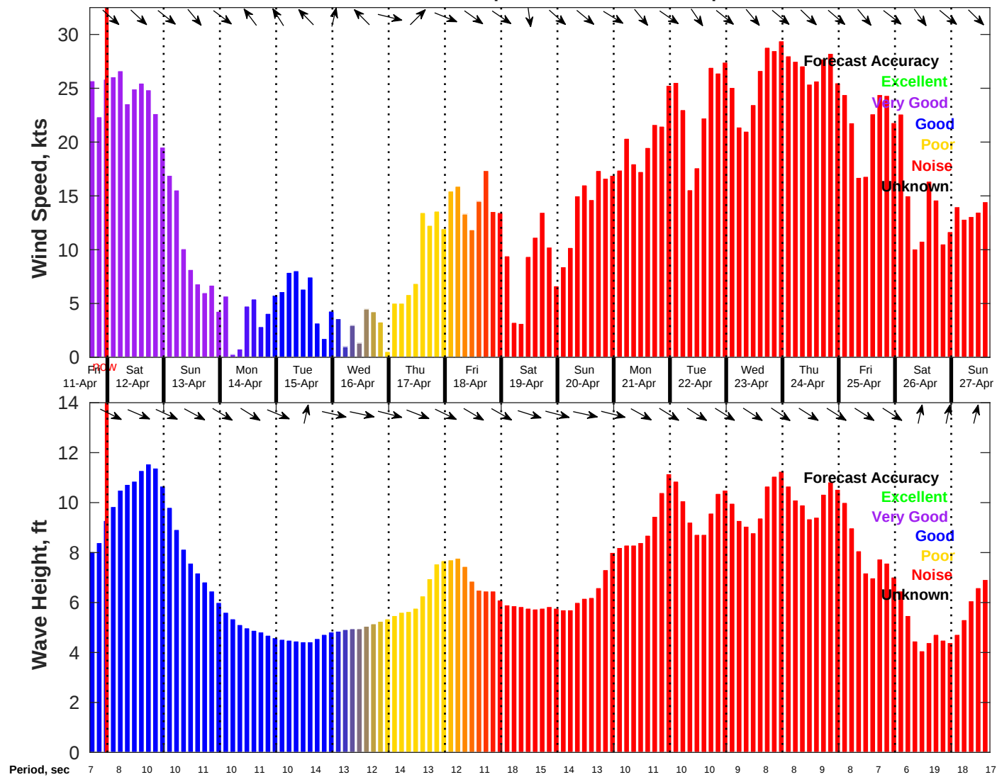
Wind & Wave Forecast for NDBC 46011 from 11-Apr-2025 16:00:00 to 27-Apr-2025 16:00:00
