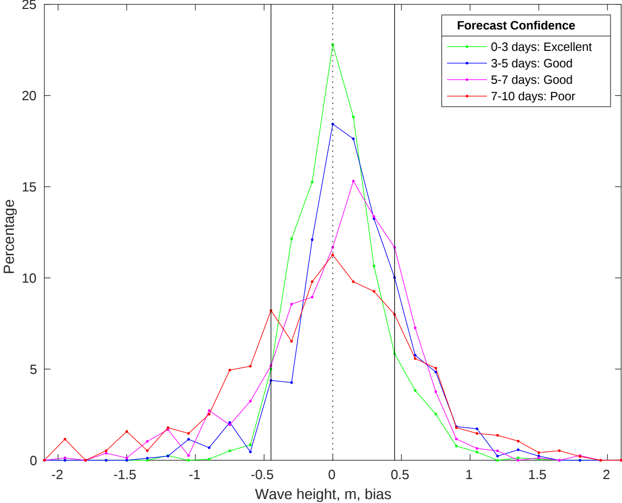
NDBC 46028 vs CMEMS Waves Bias Histogram: 12-Apr-2025
